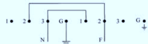
Terminal Board
