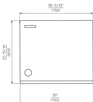
WATER-COOLED
