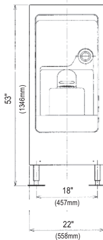
DB-130H FRONT VIEW
