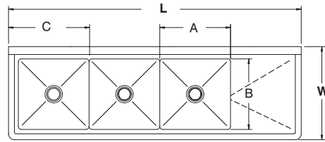
3 COMP - 1 DRBD
