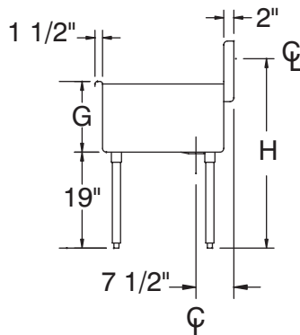
PLUMBING ROUGH-IN
