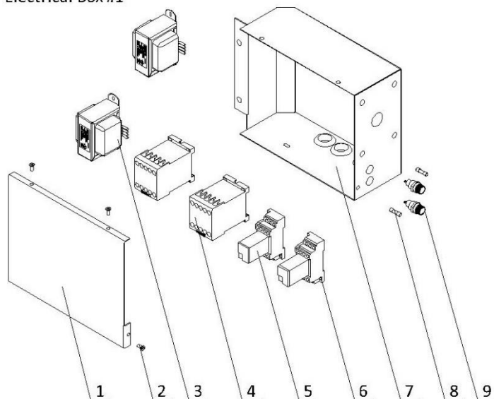
Electrical Box #1
